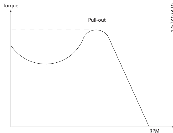
Illustration 14.1 Break-away Torque Chart
